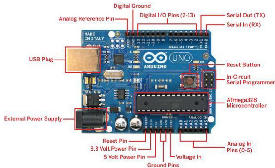
Fig 2: Arduino board
