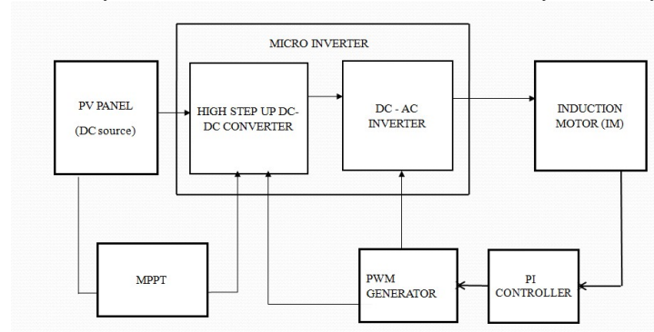
Fig1. Block Diagram of speed control of induction motor using photovoltaic micro inverter and PI controller
