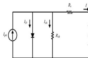
(a) Fig. 2. Thevenin's equivalent circuit derived from the single-diode model. (a) Single-diode model of a PV generator.
