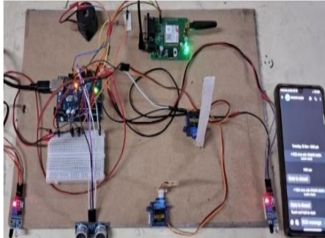
Figure 4. Hardware implementation
