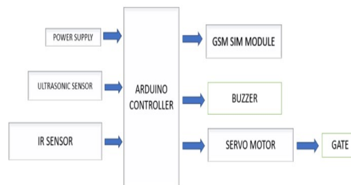
Figure 1. Block diagram Block diagram
