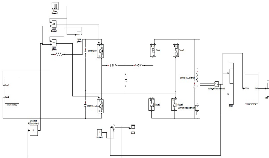
Fig. 10. Simulation circuit for proposed solar resonant converter fed PMDC motor
