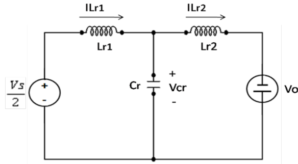
Fig. 6. Equivalent circuit for Mode I.
