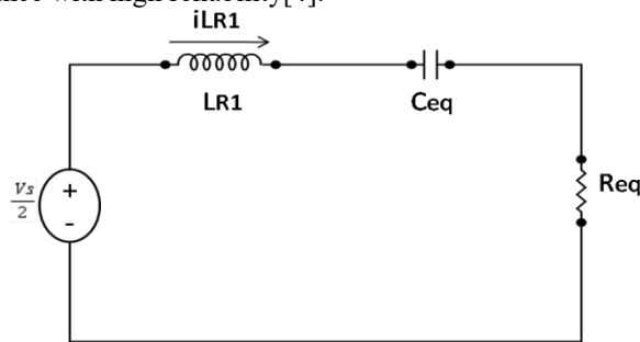
Fig. 5. Simplified equivalent circuit diagram
