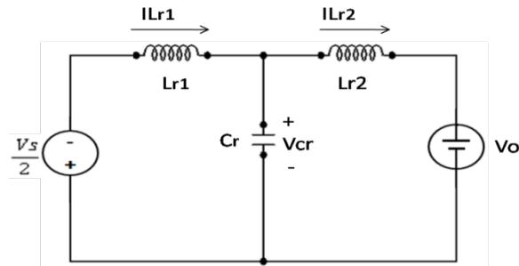
Fig.8. Equivalent circuit for Mode III.
