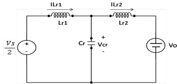
Fig. 7. Equivalent circuit for Mode II
