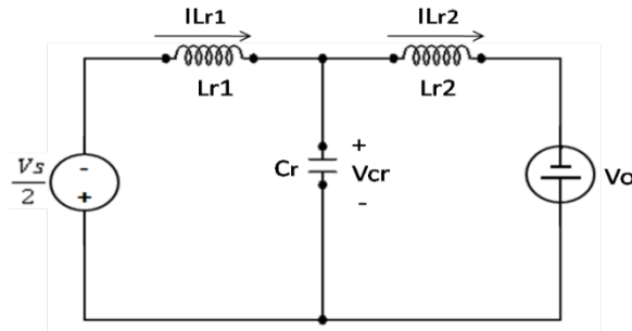
Fig. 9. Equivalent circuit for Mode IV.
