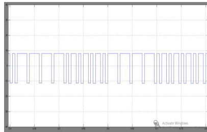
Fig. 12.Voltage after inversion
