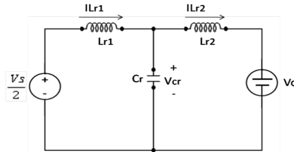
Fig. 4. Equivalent circuit for the proposed converter
