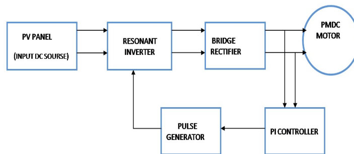
Fig. 2. Block diagram for proposed solar resonant converter fed PMDC motor
