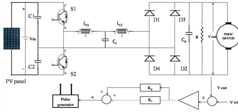
Fig.3. Circuit diagram for solar resonant converter fed PMDC motor
