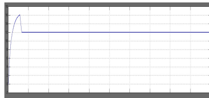
Fig. 14.Converter Output voltage
