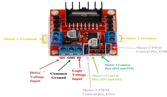
Fig-3: Motor driver L298N
