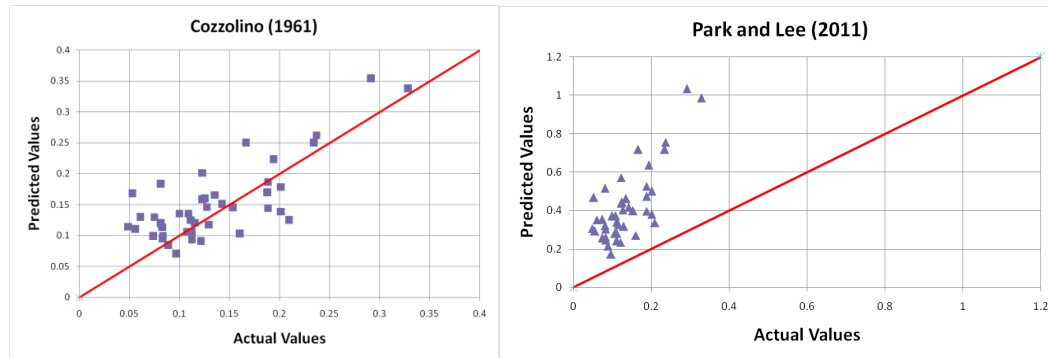
Fig. 1 Actual Compression Index, C_c versus predicted Compression Index C_c obtained by Cozzolino Model (1961) and Park and Lee Model (2011)
