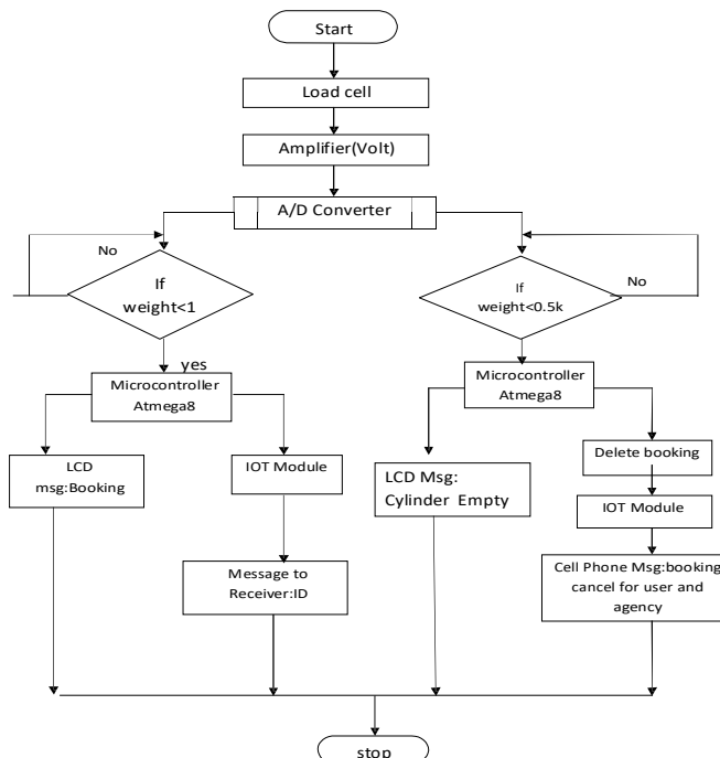
Flowchart Automatic gas booking system:
